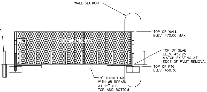
DETAIL C-C
