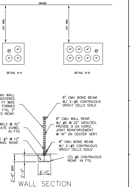
WALL SECTION
